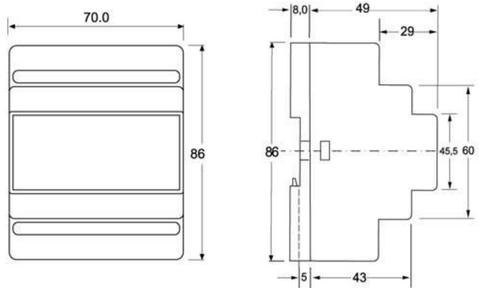
Figure 2-1. Cabinet
